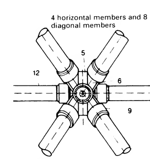
⑩ Common centre joint linking 12 members
